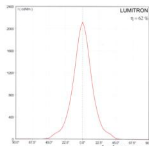
Medium Beam, MH 150W G12
