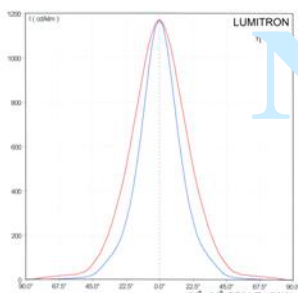
Wide Beam, MH 150W G12
