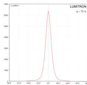
Narrow Beam, MH 150W G12
