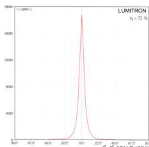
Very Narrow Beam, MH 150W G12
